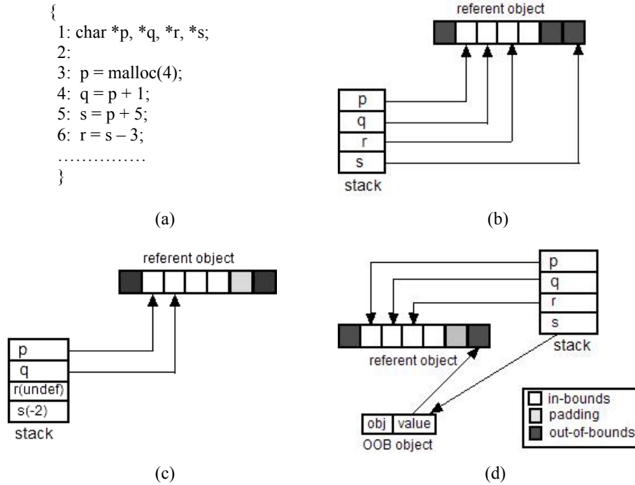
Figure 1. (a) Simple C program, memory states of (b) uninstrumented execution, (c) instrumentation with Jones and Kelly Checker, (d) instrumentation with CRED.
