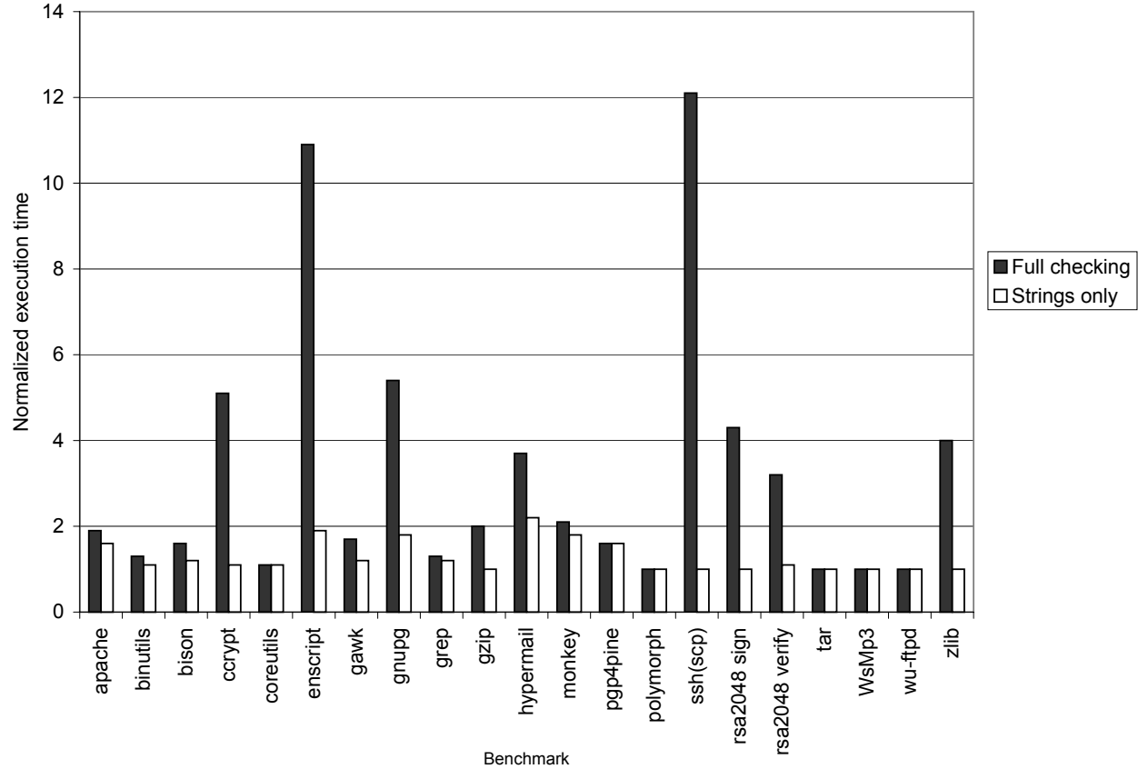
Figure 5. Performance overhead of instrumentation with and without strings only checking optimization. Non instrumented code is normalized to 1.
